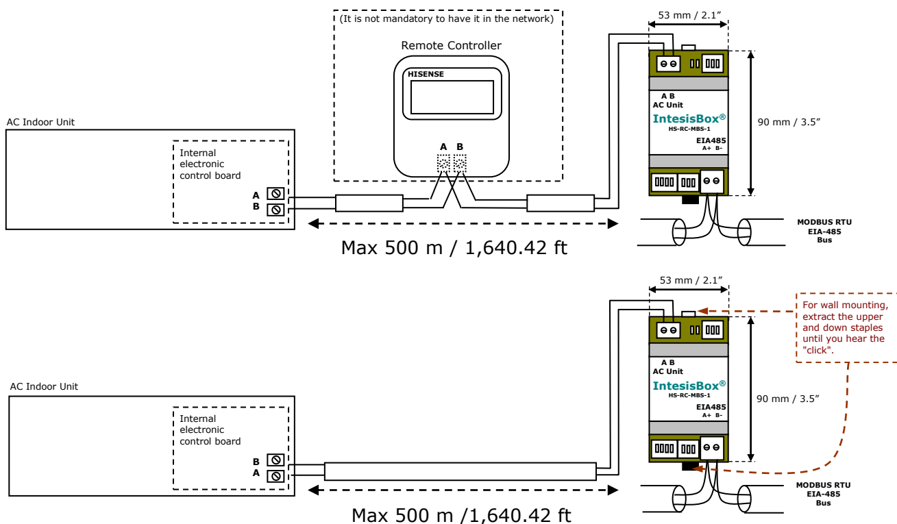
Figure 2. 1 HS-RC-MBS-1 connection diagram
