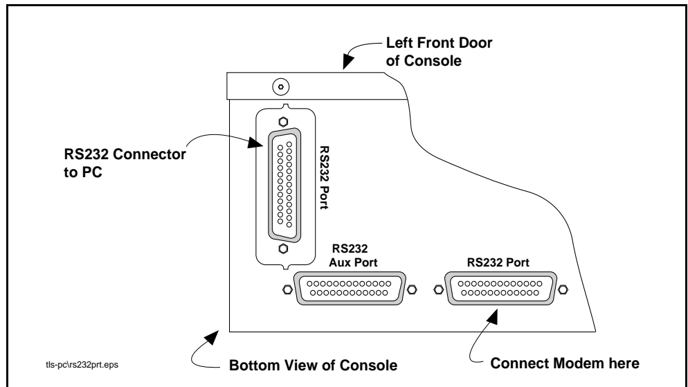
Figure 1. TLS-300-PC and TLS-300i-PC Consoles - North American Layout
